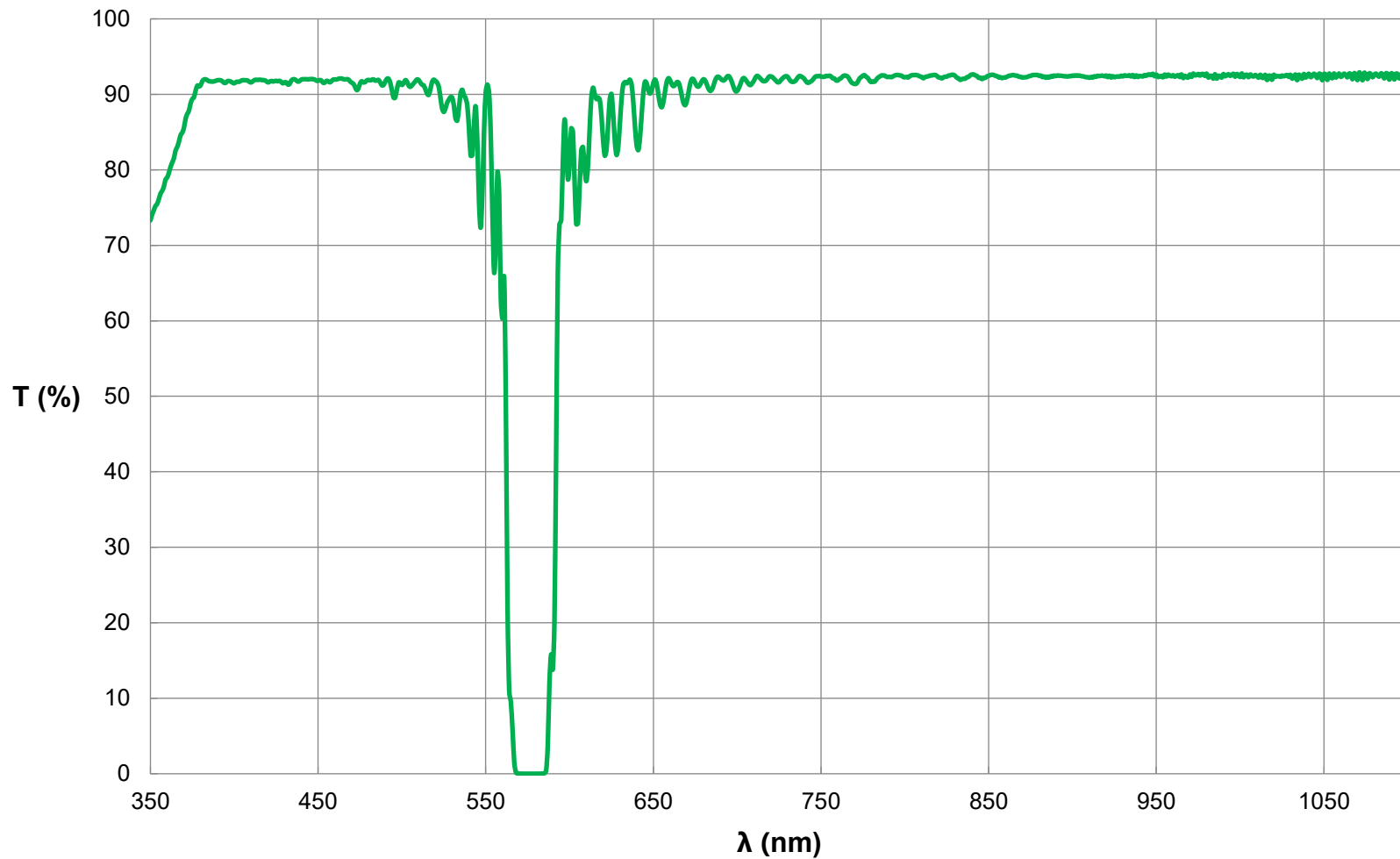
Everix Ultra-Thin OD 4 Notch Filter, 577nm, 12.5mm Diameter FOR REFERENCE ONLY
