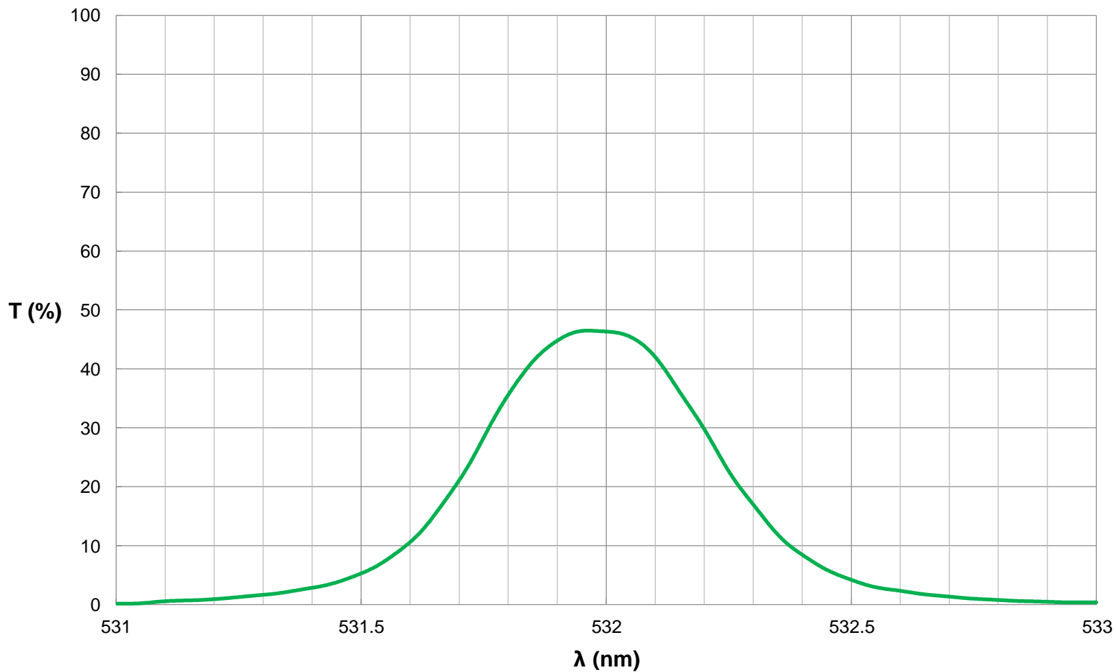
Ultra Narrow Traditional Coated Bandpass Filter, 532nm, 0.50 FWHM FOR REFERENCE ONLY
